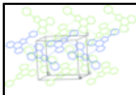
Fig. 2. A view of the crystal packing, showing the N—H···N hydrogen bonds and \pi - \pi stacking interactions. H atoms have been omitted.
