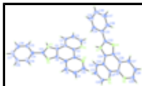
Fig. 1. The structure of (I). Displacement ellipsoids are drawn at the 30% probability level (arbitrary spheres for the H atoms).
